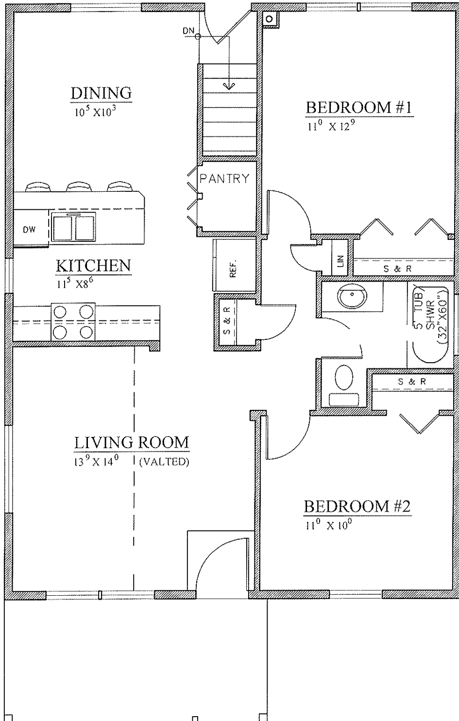
FLOOR PLAN 884 SQ. FT.
